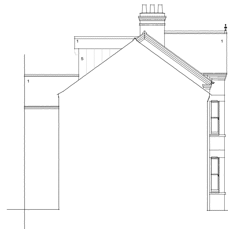
SIDE / SECTION
